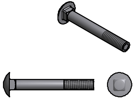
5/16 X 2 1/2" Carr Bolt (8 REQ'D)
