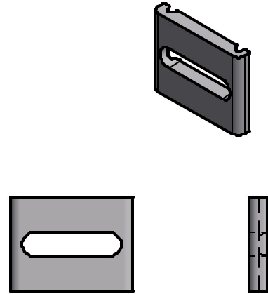
Bleacher Seat Plank Clip (24 REQ'D)
